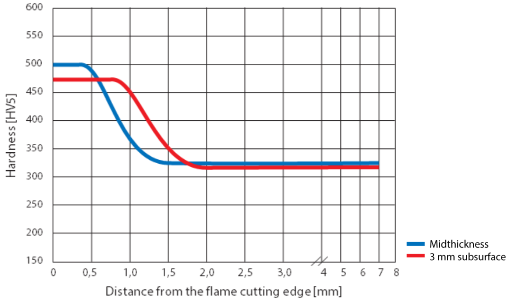
Graphic 4 Hardening of DILLIDUR 325 L at the flame cut edge
